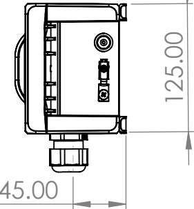
RHS VIEW
